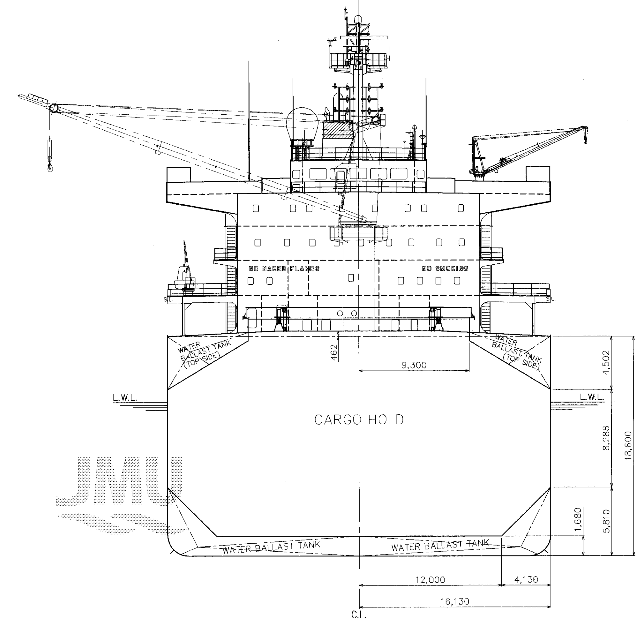
FRONT VIEW & MIDSHIP SECTION
